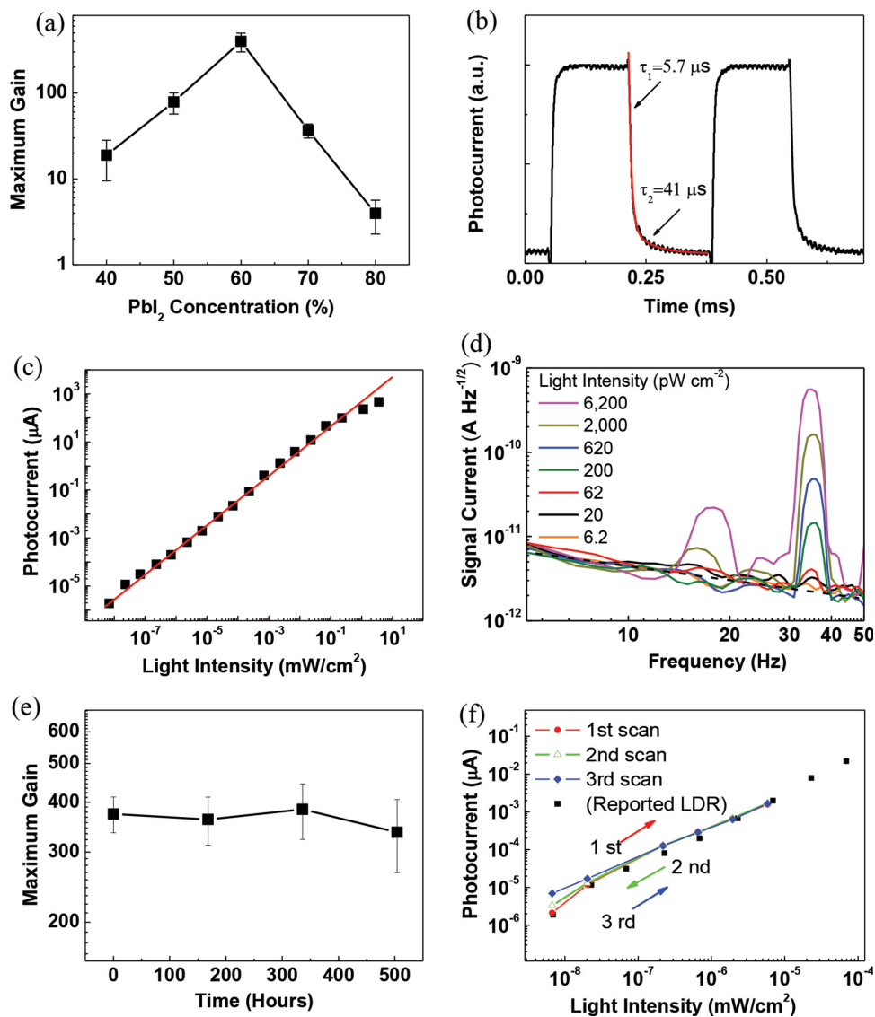
Figure 4. a) Maximum gain of the CH 3 NH 3 PbI 3 photodetectors as a function of the Pbl 2 /MAI relative mass fraction. b) Transient photocurrent of the CH 3 NH 3 PbI 3 photodetector. c) Dynamic response of the photodetector. d) The noise current spectrum of the photodetector measured with various light intensities (the dashed line is the 1/f noise background). e) The gain of the OTP photodetector measured in air at room temperature over three weeks. f) Weak light detection of the CH 3 NH 3 PbI 3 photodetector after three circles of light intensity sweeping.
